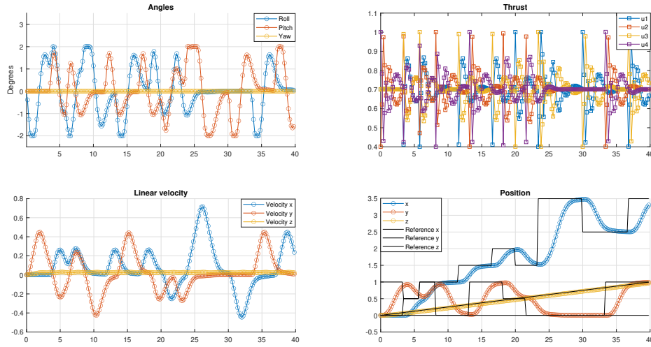
Figure 15: Response of all the sub-systems
