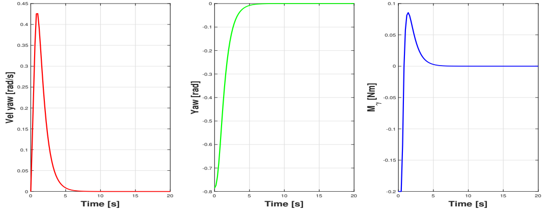
Figure 8: Regulation response of yaw dimension, starting from -\pi/4
